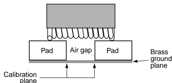
Figure 1. Test Setup
