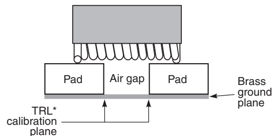
Figure 1. Test Setup
